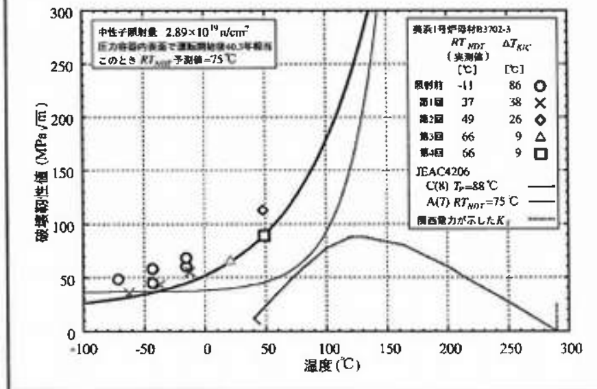
図4: PTS評価(母材B3702-3)
